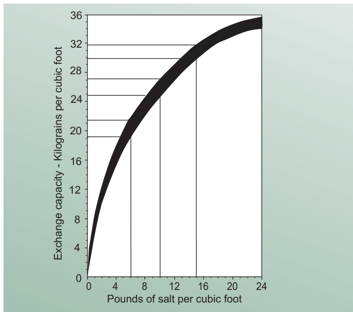
Fig. 1 Exchange capacity vs. regeneration level Sodium form C-700 Cation Resin
