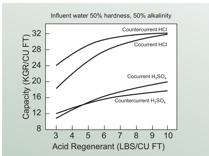
Fig. 4 Typical Aldex C-800x10H UPS Operating Capacities
