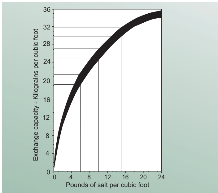
Fig. 1 Exchange capacity vs. regeneration level Sodium form C-820 Cation Resin
